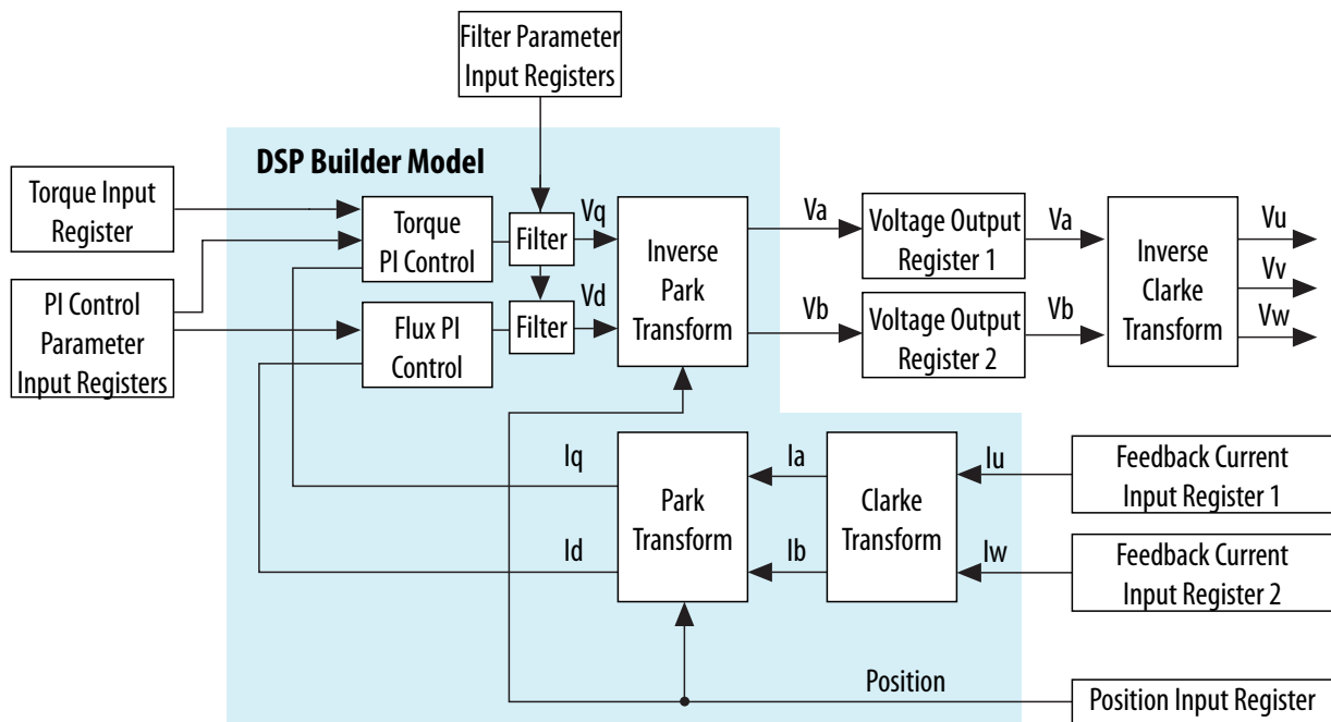
Figure 10: FOC Model integrated in Simulink with Avalon-MM Register Map (Filters for SoC Development Boards Only)
